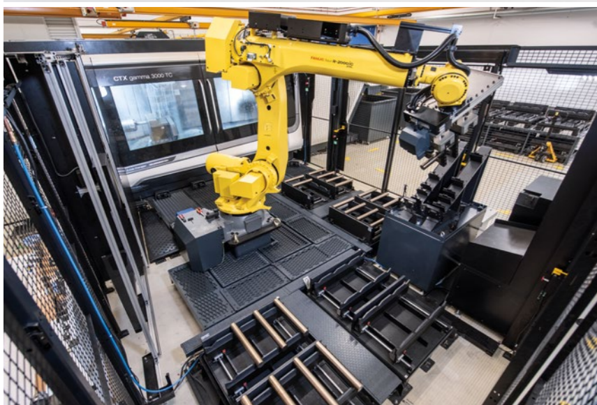
The CTX gamma 3000 TC, automated with MATRIS, produces high-precision spindles.
