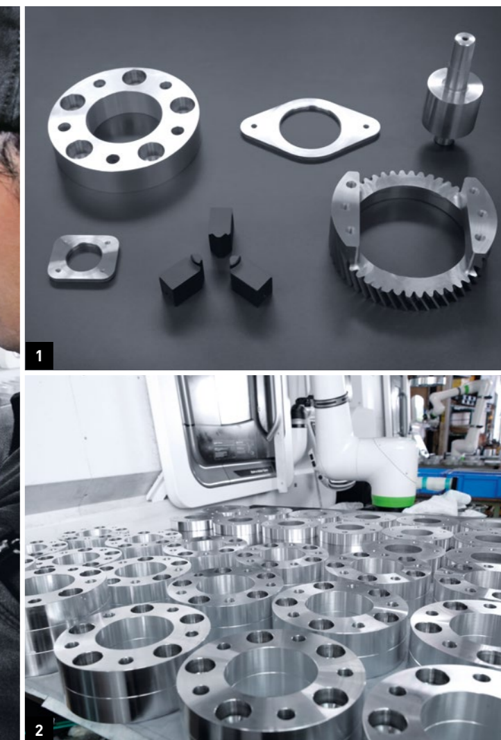
1. Main workpieces. The jaws for clamping the workpiece were also designed in-house. 2. Workpieces are stacked for long hours of continuous operation.
