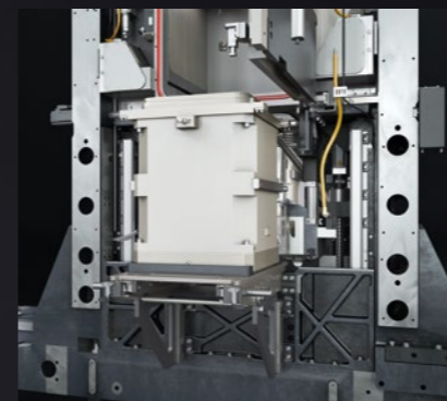
Exchangeable build container for reduced job-to-job time
